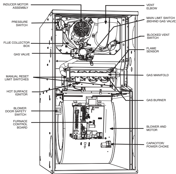
Fig. 1 – 80% AFUE Single Stage Furnace Components A10259
